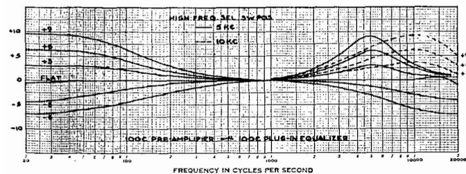
FIG. 9(a). Frequency response curves of combination of preamplifier and equalizer.
