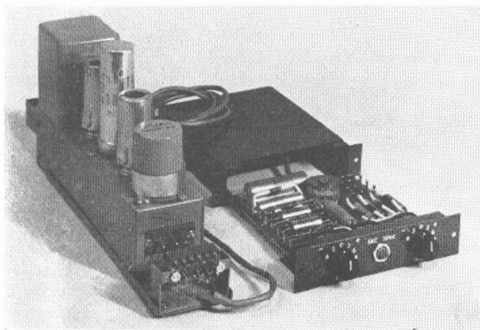
FIG. 10. Model 100D preamplifier and Model 100B plug-in equalizer package.
