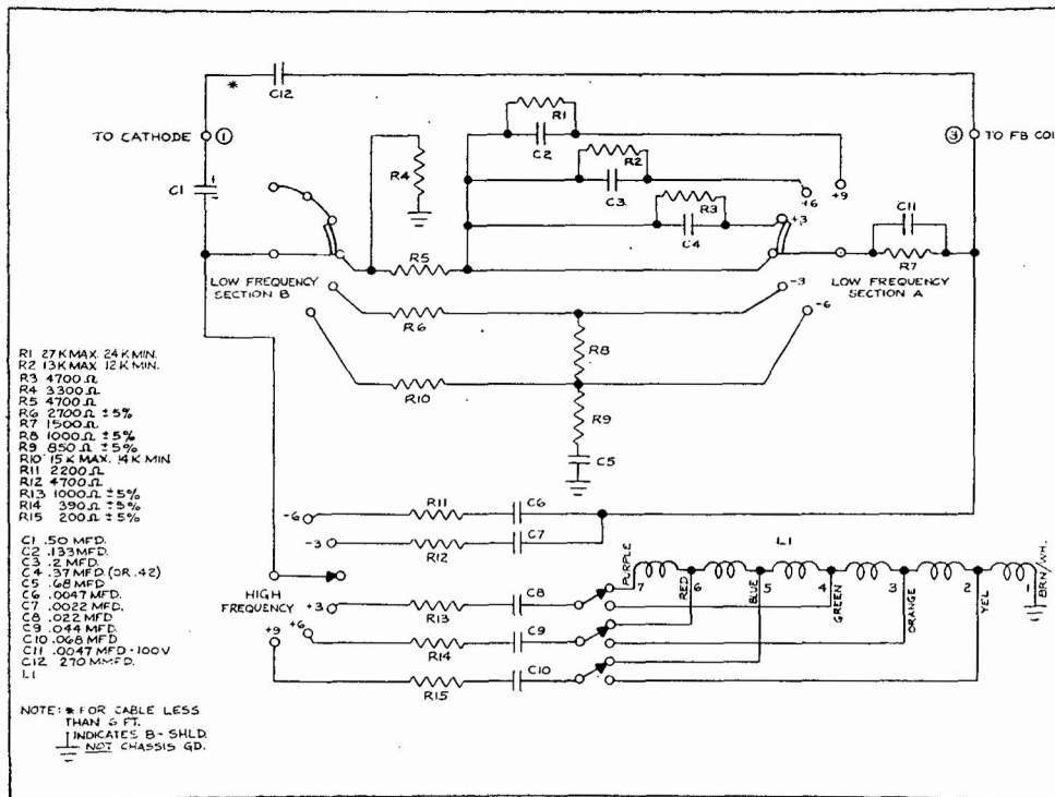
FIG. 9(b). Schematic of Model 108B equalizer.
