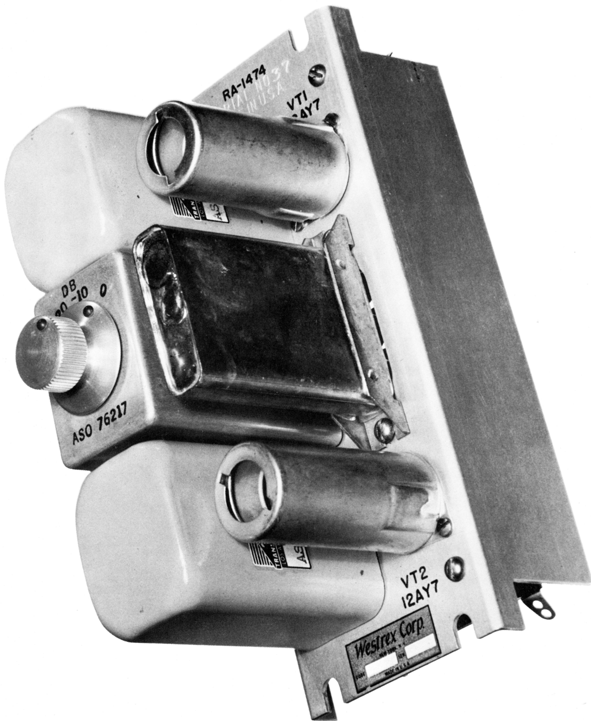
Figure 1 View of RA-1474-A Amplifier with Plug-in Unit
