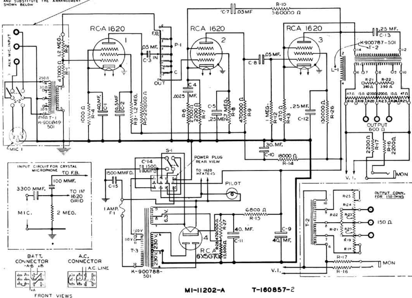
Figure 3—Schematic Diagram
