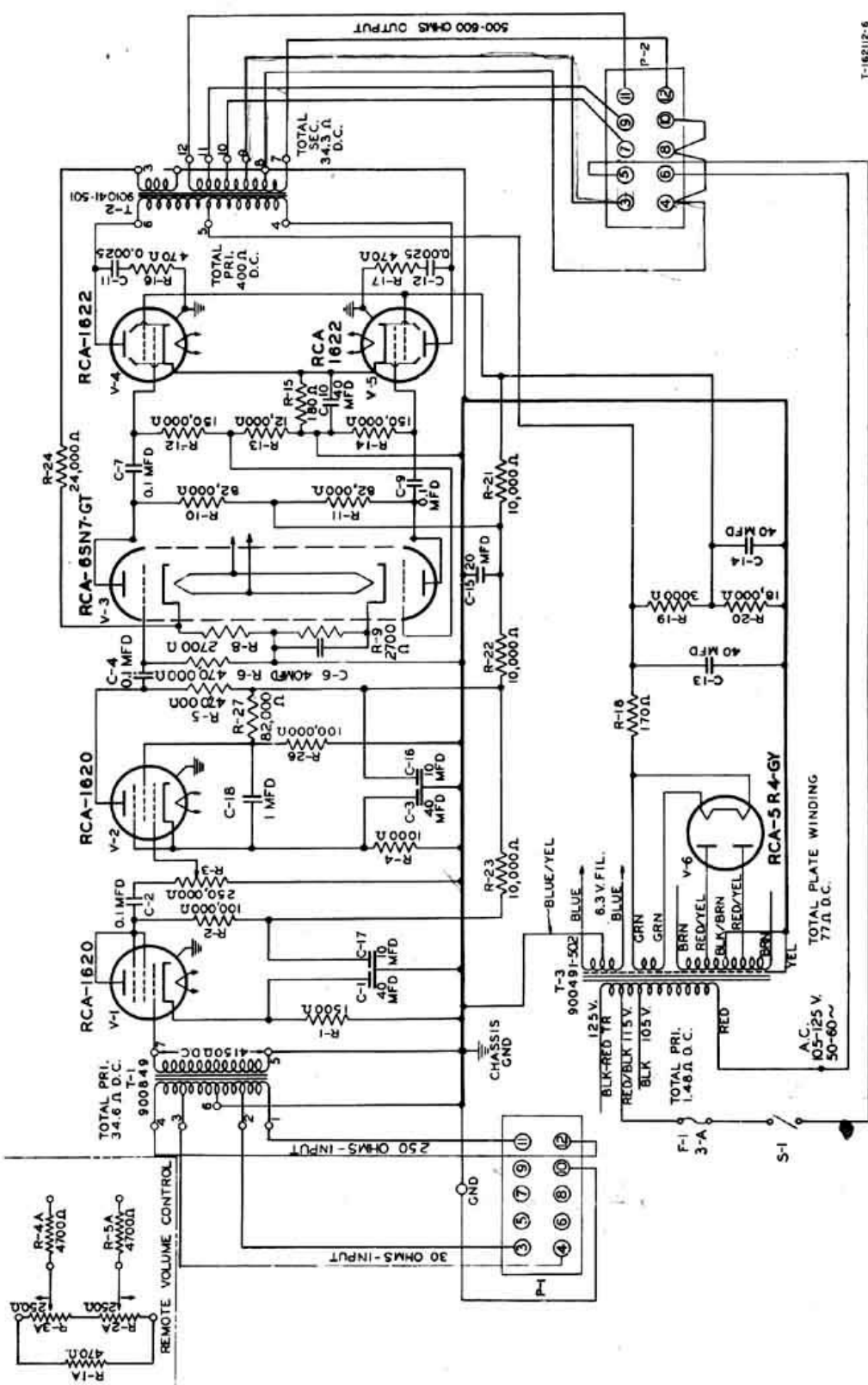
Figure 2—Schematic diagram of BA-4C.
