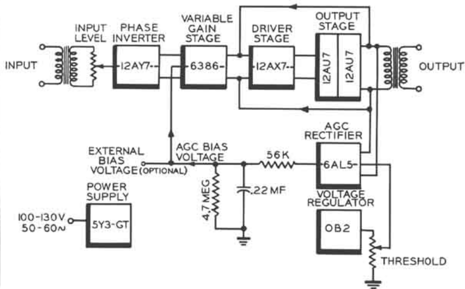
FIG. 2. Simplified block diagram of AGC program amplifier. Use of external bias source permits automatic fading or remote gain control.
