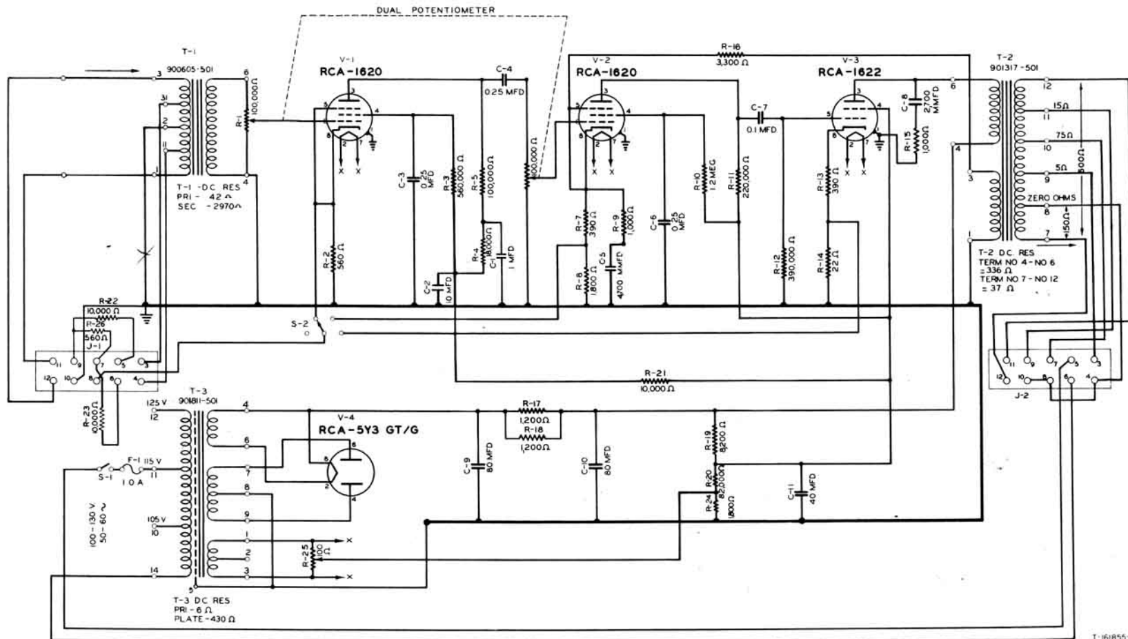
Figure 2—Schematic diagram of Type BA-3C Program Amplifier.
