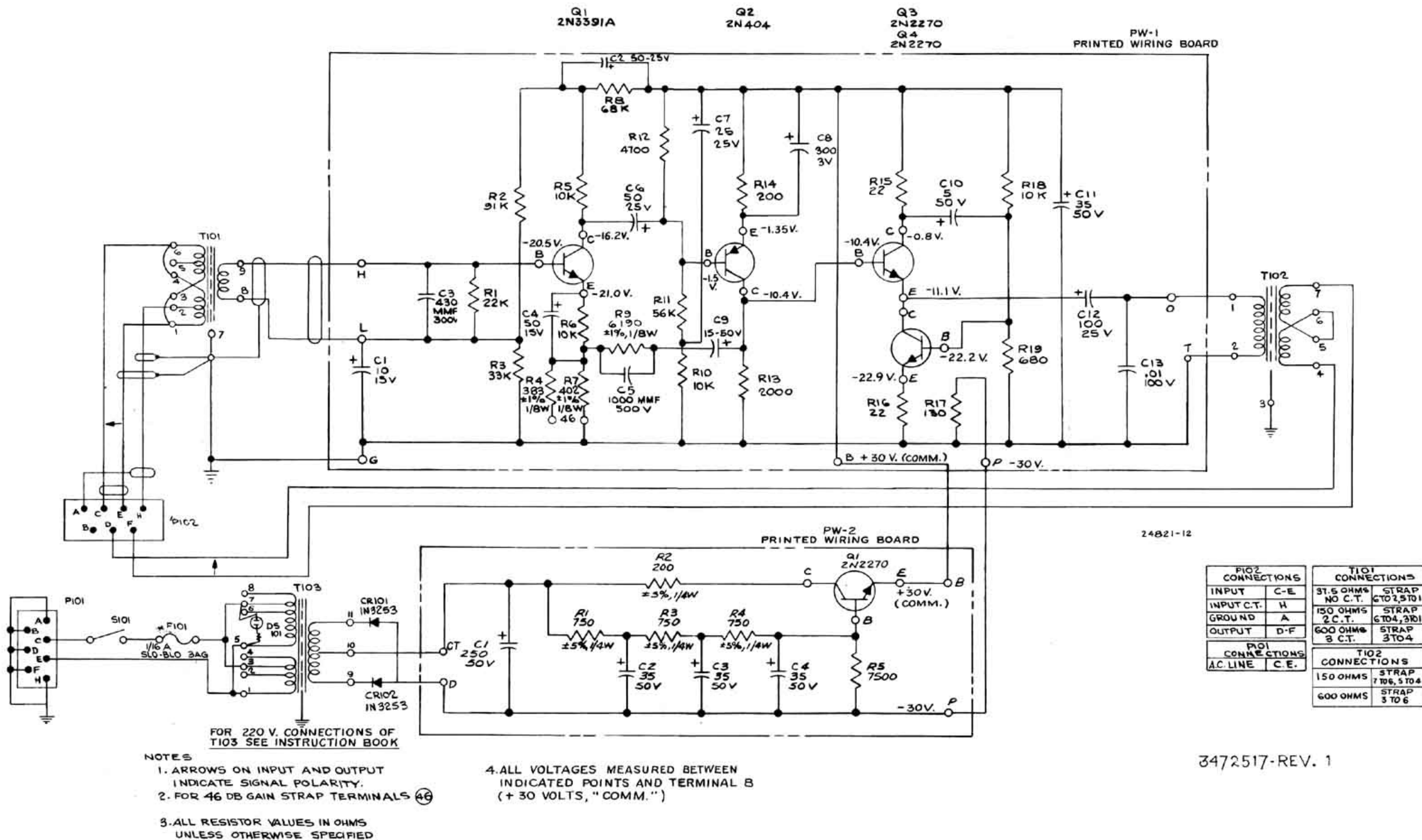
Figure 12—Schematic Diagram
