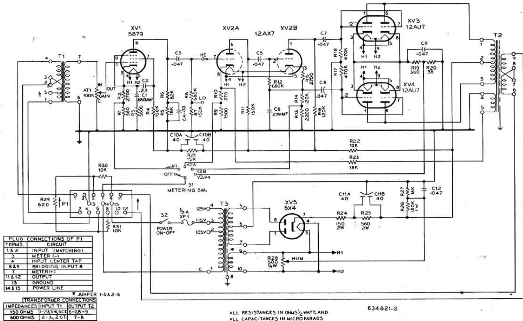
Figure 4 - Schematic Diagram
