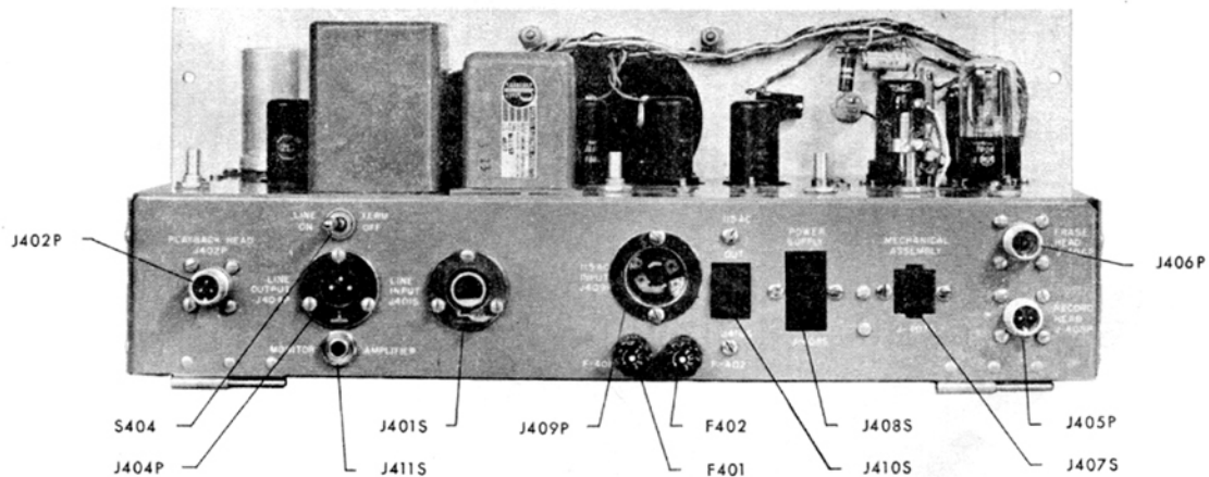
ELECTRONIC ASSEMBLY TOP & REAR VIEWS CATALOG NO. 5701 AMPEX CORPORATION REDWOOD CITY, CALIFORNIA
